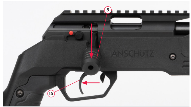
Fig. 30 Closing the bolt
