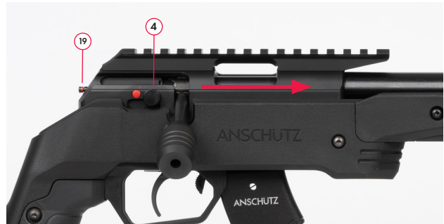
Fig. 18 Safety catch "ready to fire" (red dot visible)
