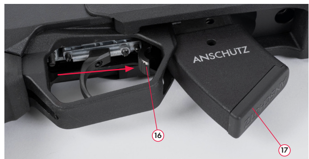
Fig. 27 Pushing the magazine release lever forward
