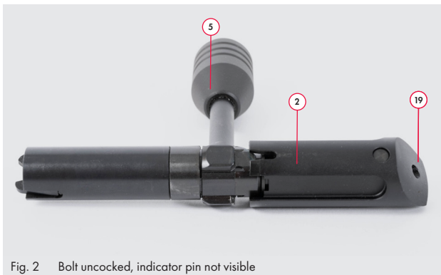
Fig. 2 Bolt uncocked, indicator pin not visible
